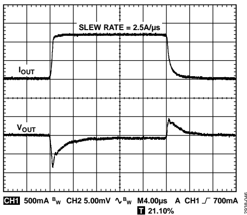
Figure 44. Output Transient Response, V_{OUT} = 3.3\text{ V} , C_{OUT} = 10\ \mu\text{F} , Channel 1 = Load Current, Channel 2 = V_{OUT}
