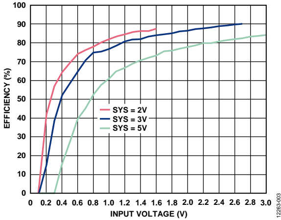
Figure 3. Efficiency vs. Input Voltage, I_{IN} = 10 \mu\text{A}
