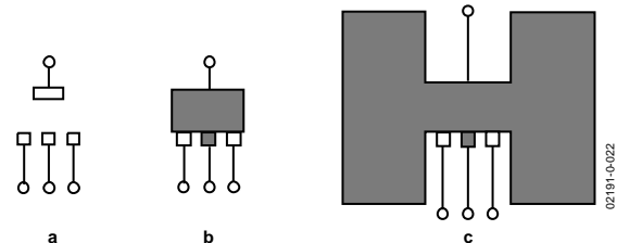
Figure 22. PCB Layouts
