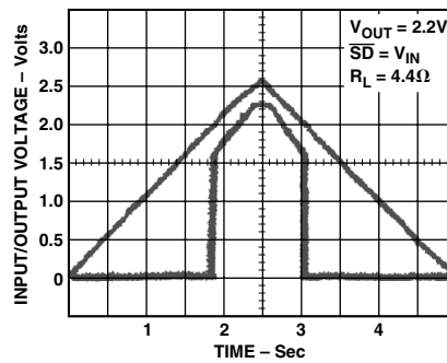
Figure 9. Power-Up/Power-Down
