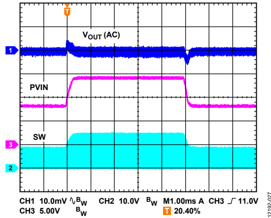
Figure 27. Line Transient Response, V_{PVIN} from 8 V to 14 V, I_{OUT} = 12\text{ A}
