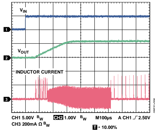
Figure 56. Startup, V_{OUT} = 1.2\text{ V} , 10 mA, V_{IN} = 5\text{ V}
