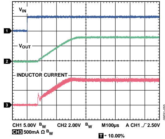
Figure 55. Startup, V_{OUT} = 3.3\text{ V} , 800 mA
