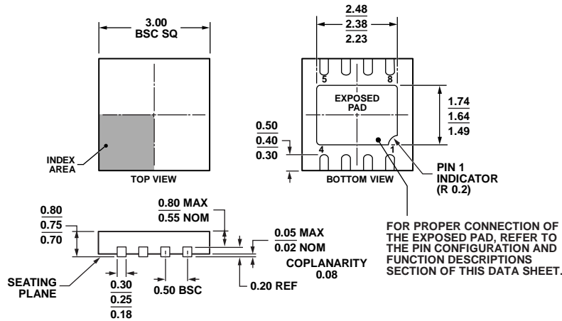
Figure 93. 8-Lead Lead Frame Chip Scale Package [LFCSP] (CP-8-5) Dimensions shown in millimeters
