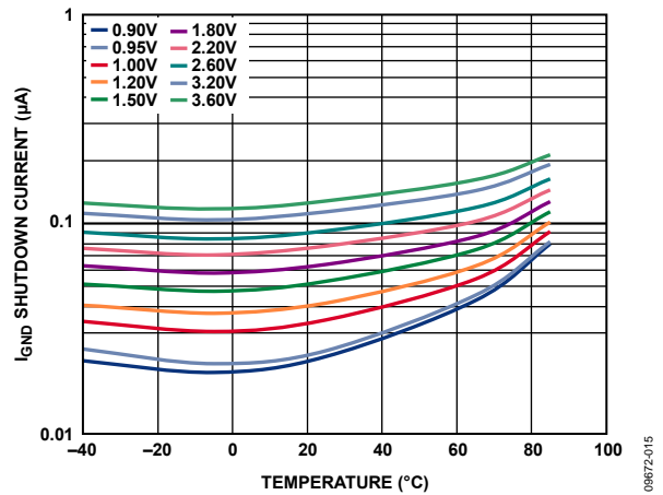
Figure 15. Ground Shutdown Current vs. Temperature, V_{OUT} = 0\text{ V} , Different Input Voltage ( V_{IN} )
