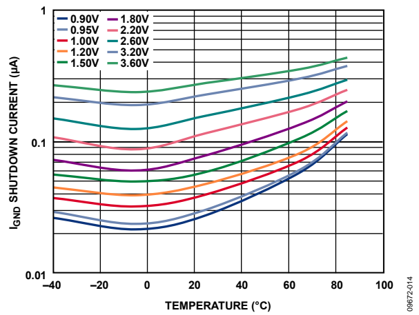
Figure 14. Ground Shutdown Current vs. Temperature, Output Open, Different Input Voltage ( V_{IN} )
