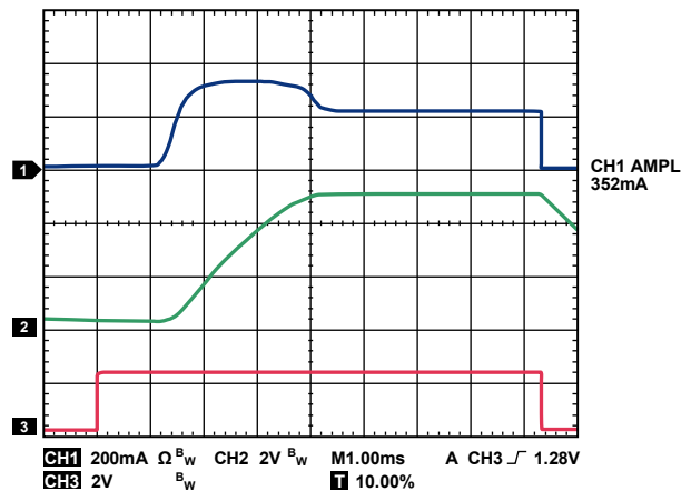
Figure 30. Typical Rise Time and Inrush Current, C_{LOAD} = 100\ \mu\text{F} , V_{IN} = 5.5\text{ V} , I_{LOAD} = 350\text{ mA}
