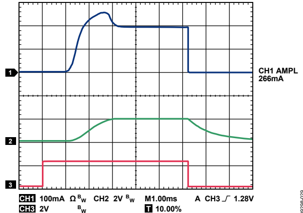
Figure 29. Typical Rise Time and Inrush Current, C_{LOAD} = 100\ \mu\text{F} , V_{IN} = 1.9\text{ V} , I_{LOAD} = 270\text{ mA}
