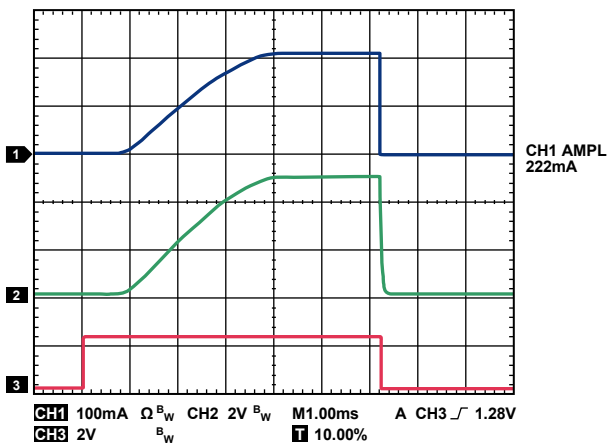
Figure 28. Typical Turn-On Delay Time with V_{IN} = 5.5\text{ V} , I_{LOAD} = 220\text{ mA}
