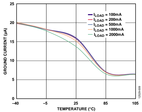
Figure 9. Ground Current vs. Temperature, Different Load Currents, V IN = 6.5 V
