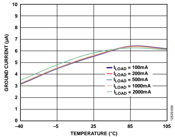
Figure 8. Ground Current vs. Temperature, Different Load Currents, V IN = 2.3 V
