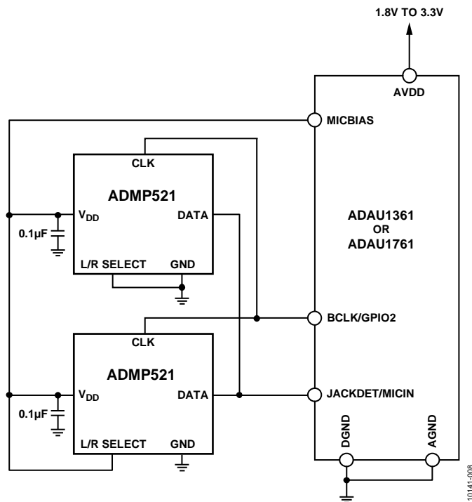
Figure 14. ADAU1361 or ADAU1761 Stereo Interface Block Diagram
