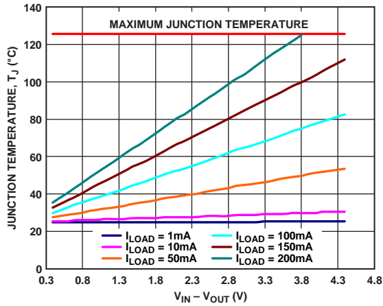
Figure 43. TSOT, 500 mm 2 of PCB Copper, T A = 25°C
