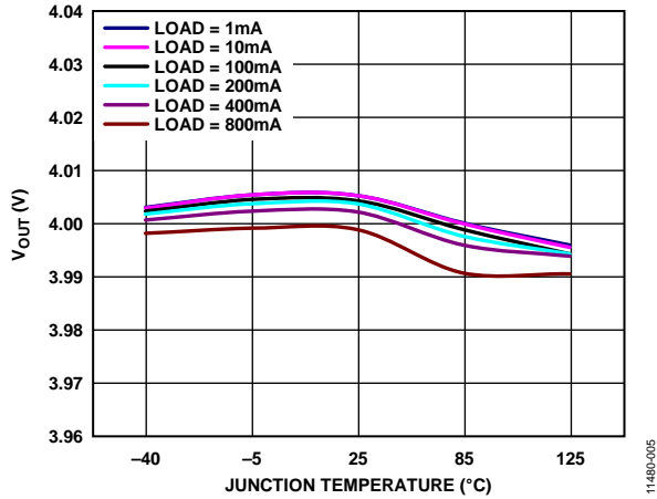
Figure 5. Output Voltage ( V_{OUT} ) vs. Junction Temperature ( T_J ), ADM7151-02, V_{OUT} = 4\text{ V}
