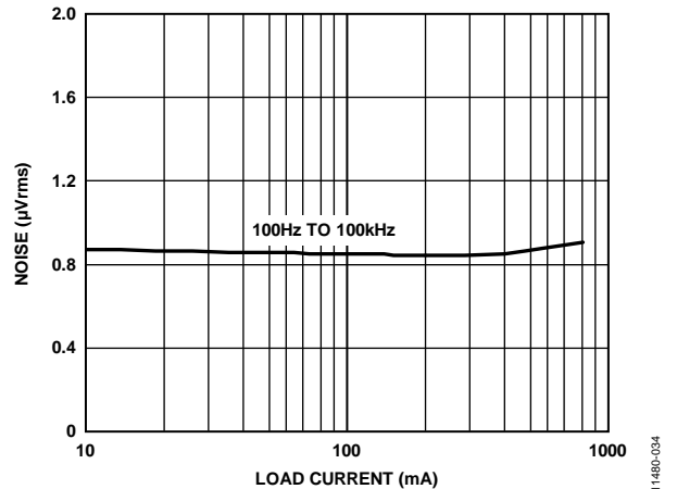
Figure 34. RMS Output Noise vs. Load Current ( I_{LOAD} ), 100 Hz to 100 kHz, ADM7151-02, V_{OUT} = 4\text{ V}
