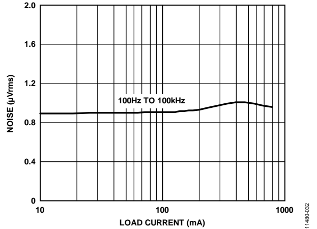
Figure 32. RMS Output Noise vs. Load Current ( I_{LOAD} ), 100 Hz to 100 kHz, ADM7151-04, V_{OUT} = 5\text{ V}
