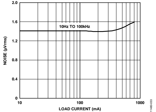
Figure 33. RMS Output Noise vs. Load Current ( I_{LOAD} ), 10 Hz to 100 kHz, ADM7151-02, V_{OUT} = 4\text{ V}
