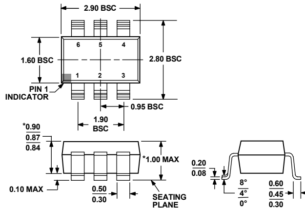
Figure 34. 6-Lead Thin Small Outline Transistor Package [TSOT] (UJ-6)
