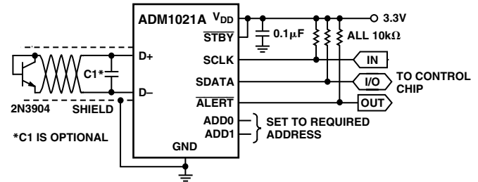
Figure 8. Typical Application Circuit
