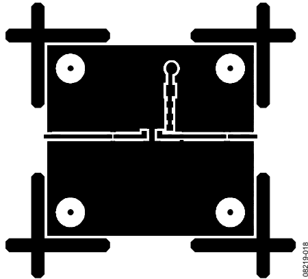
Figure 19. Evaluation Board Layout (Top)
