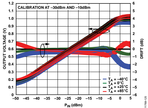
Figure 25. Distribution of Log Conformance Error with Respect to V_{LOG} at 2700 MHz vs. P_{IN} and Temperature at 2700 MHz
