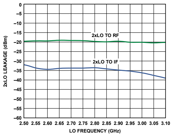
Figure 33. 2xLO Leakage vs. LO Frequency
