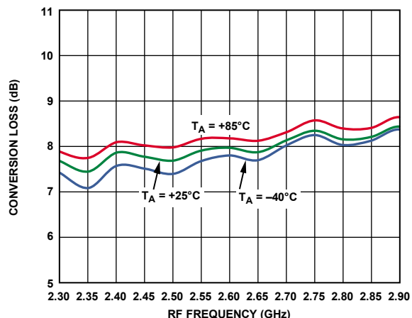
Figure 4. Power Conversion Loss vs. RF Frequency
