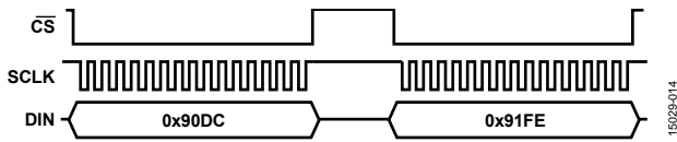
Figure 33. SPI Sequence for Writing 0xFEDC to XG_BIAS_LOW
