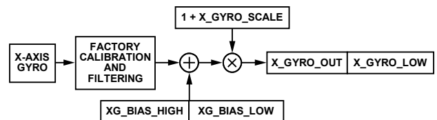
Figure 43. User Calibration Signal Path, Gyroscopes
