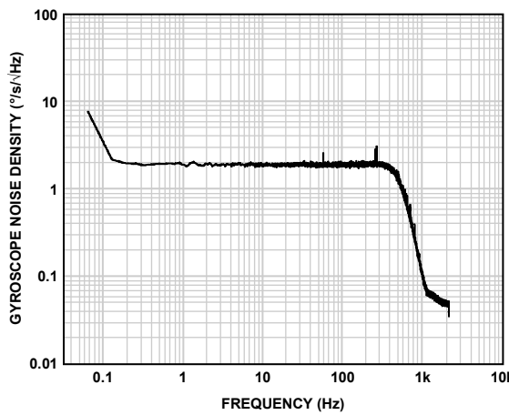
Figure 12. Gyroscope Noise Density, T C = 25°C
