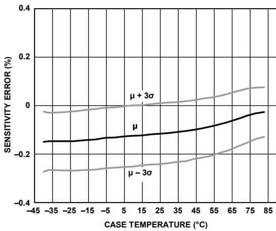
Figure 9. Gyroscope Sensitivity Error, +85°C to -40°C, 1°C/min
