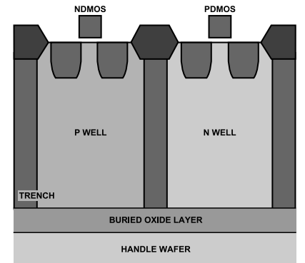
Figure 51. Trench Isolation
