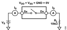
Figure 37. Switch Unpowered Leakage
