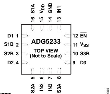
Figure 4. ADG5233 LFCSP_WQ Pin Configuration
