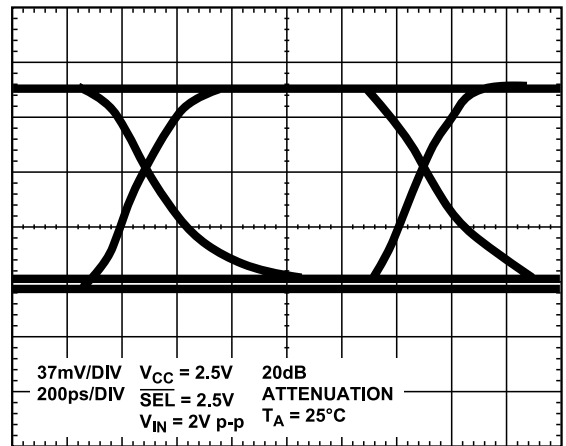
Figure 23. Eye Pattern; 1 Gbps, V_{CC} = 2.5 \text{ V} , PRBS 31
