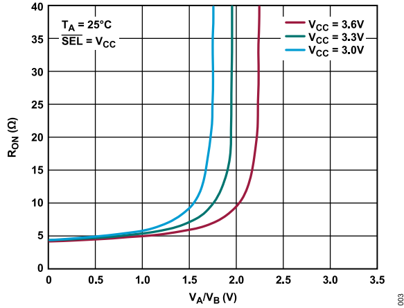
Figure 3. On Resistance vs. Input Voltage, V_{CC} = 3.0\text{ V} , 3.3\text{ V} , and 3.6\text{ V}
