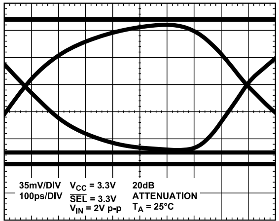
Figure 22. Eye Pattern; 1.244 Gbps, V_{CC} = 3.3 \text{ V} , PRBS 31
