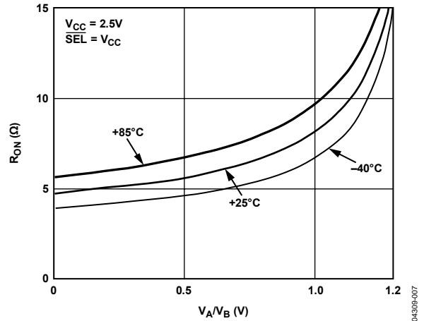
Figure 8. On Resistance vs. Input Voltage for Different Temperatures
