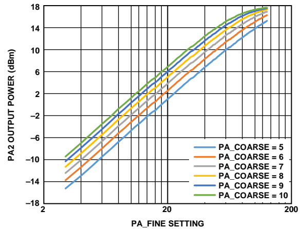
Figure 42. PA2 Output Power vs. PA_FINE Setting and PA_COARSE Setting with PA_FINE on a Logarithmic Scale, PAOLDO_VOUT_CON=15, RF Frequency = 460 MHz, V_{DD} = 3.0 V , T_A = 25^\circ C
