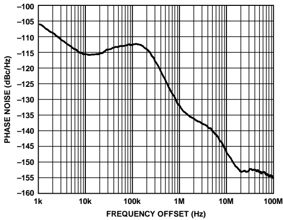
Figure 39. Phase Noise vs. Frequency Offset, RF Frequency = 460 MHz, PA2 Output Power = 17 dBm, V_{DD} = 3.0 V , T_A = 25^\circ C
