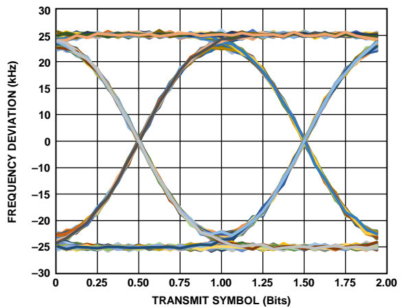
Figure 44. Transmit Eye Diagram; PA2 Output Power = 17 dBm; Configuration 460 MHz/7.2 kbps; BT = 0.5; V_{DD} = 3.0 V ; T_A = 25^\circ C
