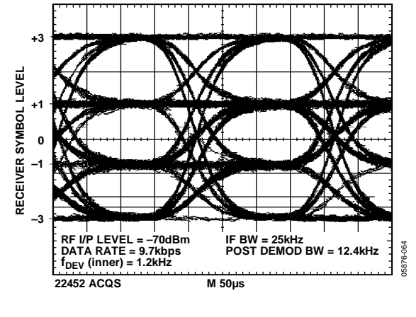
Figure 28. 4FSK Receiver Eye Diagram Measure Using the Test DAC Output
