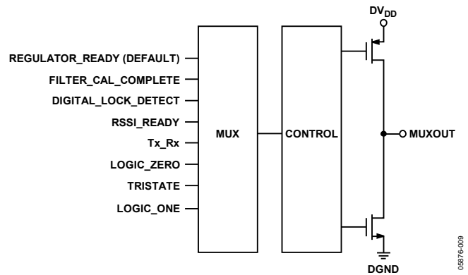
Figure 35. MUXOUT Circuit
