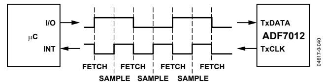
Figure 31. TxCLK/TxDATA Synchronization.
