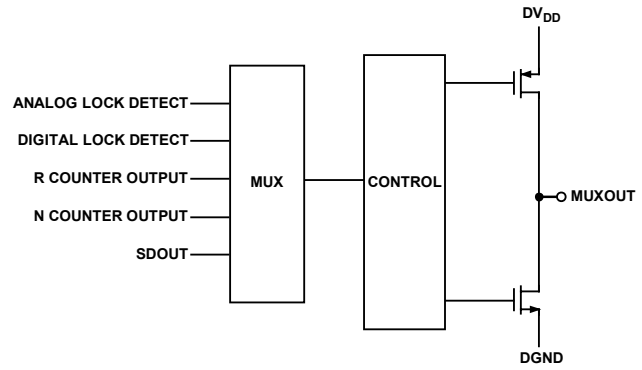
Figure 15. MUXOUT Circuit
