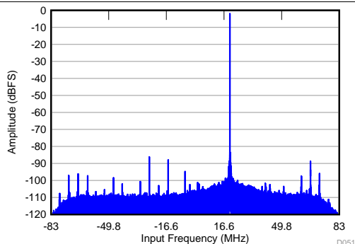
f_{IN} = 1.78 \text{ GHz} , A_{IN} = -2 \text{ dBFS} , f_S = 2949.12 \text{ MSPS} , SNR = 64 dBFS, SFDR (includes IL) = 83 dBc
