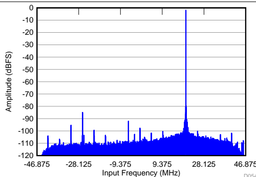
f_{IN} = 1.78 \text{ GHz} , A_{IN} = -2 \text{ dBFS} , f_S = 2949.12 \text{ MSPS} , SNR = 64.5 dBFS, SFDR (includes IL) = 79 dBc
