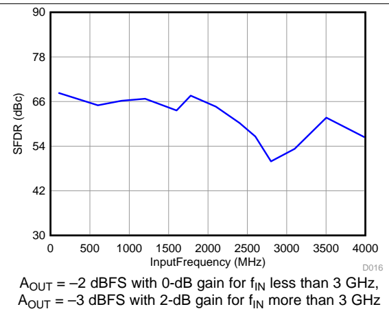
Figure 37. Spurious-Free Dynamic Range vs Input Frequency
