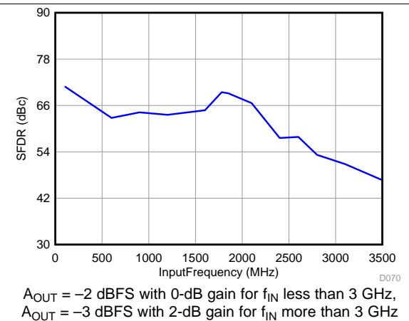
Figure 38. Spurious-Free Dynamic Range vs Input Frequency ( f_s = 2457.6 MSPS)
