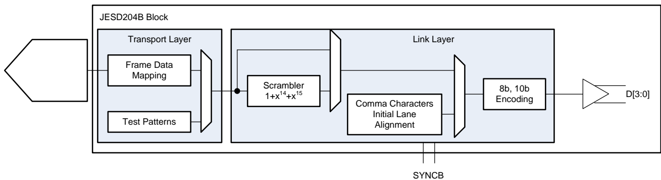
Figure 133. JESD Digital Block Implementation
