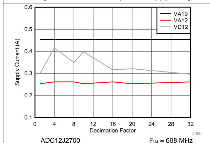
Figure 23. Supply Current vs Decimation Setting
