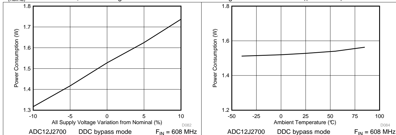
Figure 21. Power Consumption vs Supply Voltage
