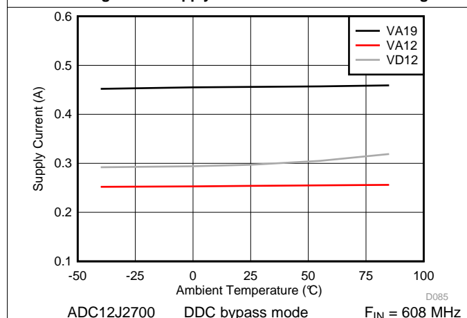
Figure 25. Supply Current vs Temperature
