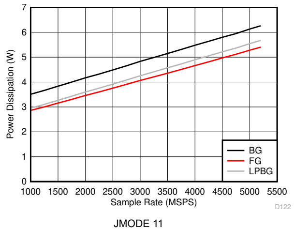
Figure 6-138. Dual Channel Mode: Power Dissipation vs Sample Rate
