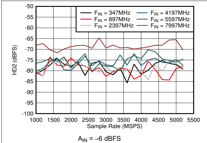
Figure 6-51. Dual Channel Mode: HD2 vs Sample Rate and Input Frequency
