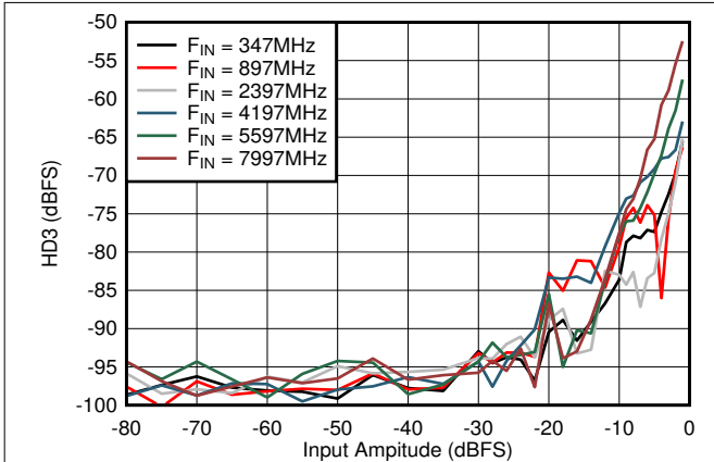
Figure 6-63. DES Mode: HD3 vs Input Amplitude and Frequency
