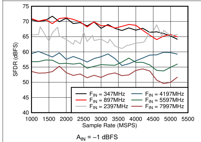
Figure 6-47. Dual Channel Mode: SFDR vs Sample Rate and Input Frequency
