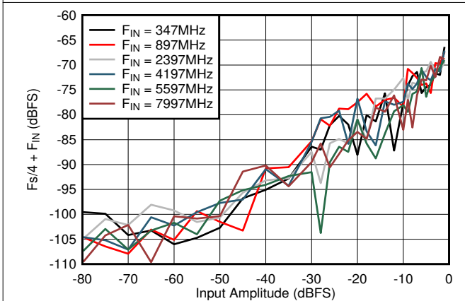
Figure 6-67. DES Mode: F_s/4 + F_{IN} vs Input Amplitude and Frequency
