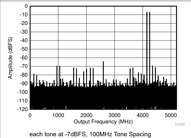
Figure 6-14. DES Mode: Two Tone FFT at 4197MHz
