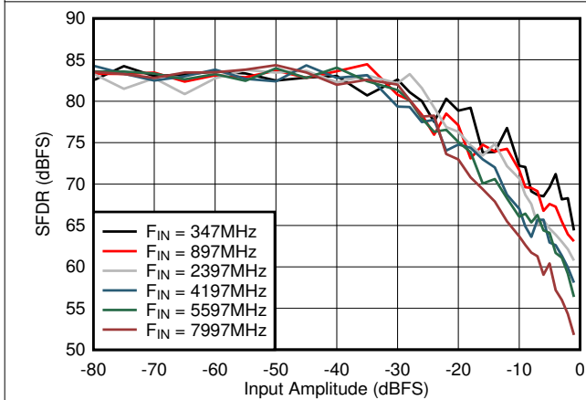
Figure 6-59. DES Mode: SFDR vs Input Amplitude and Frequency
