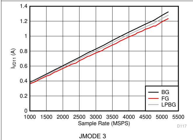
Figure 6-133. Dual Channel Mode: I_{VD11} vs Sample Rate
