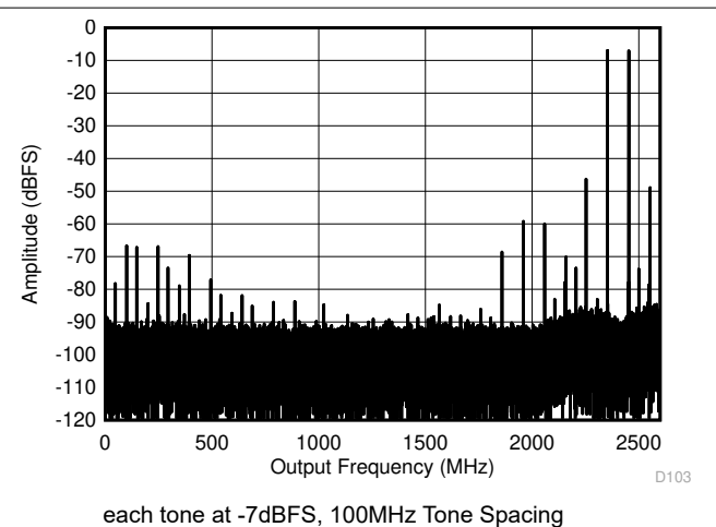
Figure 6-28. DES Mode: Two Tone FFT at 7997MHz
