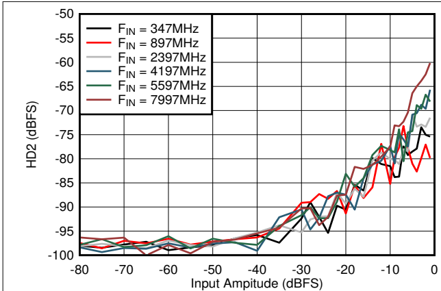
Figure 6-75. Dual Channel Mode: HD2 vs Input Amplitude and Frequency
