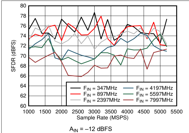
Figure 6-49. Dual Channel Mode: SFDR vs Sample Rate and Input Frequency
