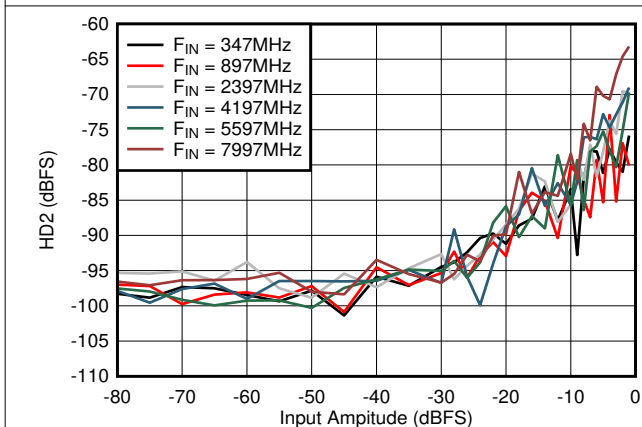
Figure 6-61. DES Mode: HD2 vs Input Amplitude and Frequency
