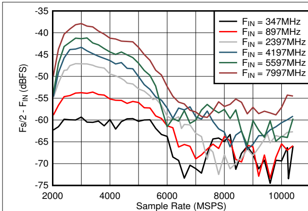
Figure 6-41. DES Mode: F_s/2 - F_{IN} vs Sample Rate and Input Frequency
