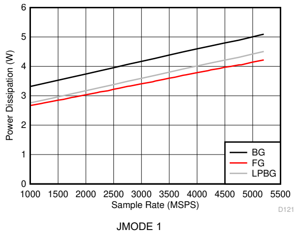
Figure 6-137. Dual Channel Mode: Power Dissipation vs Sample Rate
