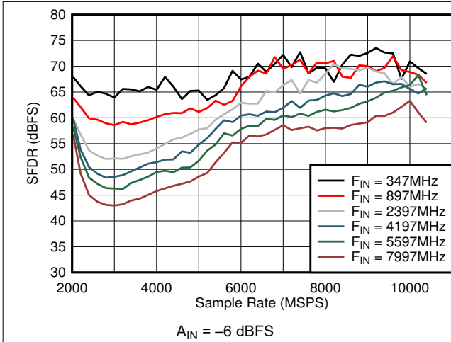
Figure 6-33. DES Mode: SFDR vs Sample Rate and Input Frequency
