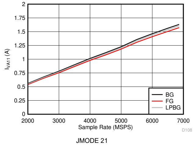
Figure 6-124. DES Mode: I_{VA11} vs Sample Rate
