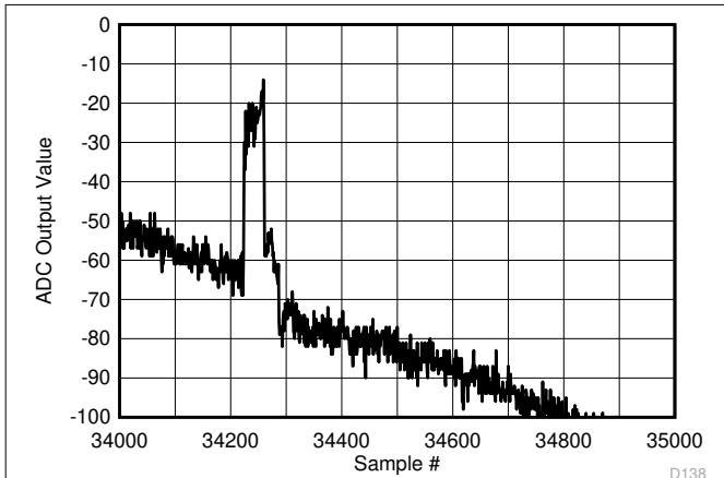
Figure 6-143. Background Calibration Core Transition (AC Signal - zoomed)
