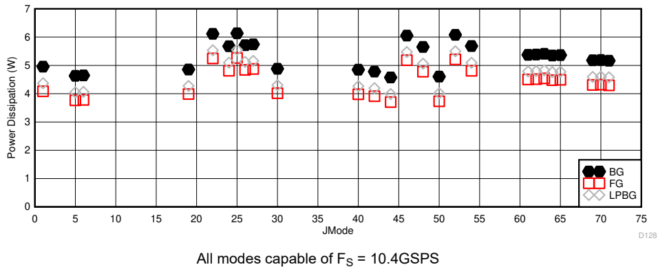
Figure 6-112. DES Mode: Power Dissipation vs JMODE at 10.4GSPS
