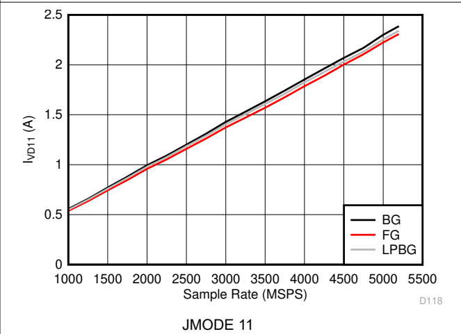
Figure 6-134. Dual Channel Mode: I_{VD11} vs Sample Rate
