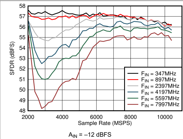
Figure 6-34. DES Mode: SFDR vs Sample Rate and Input Frequency
