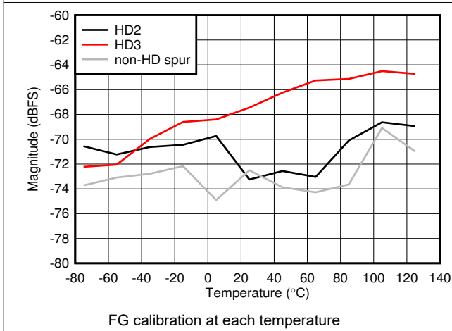
Figure 6-91. Dual Channel Mode: HD2, HD3 and Worst non-HD Spur vs Temperature
