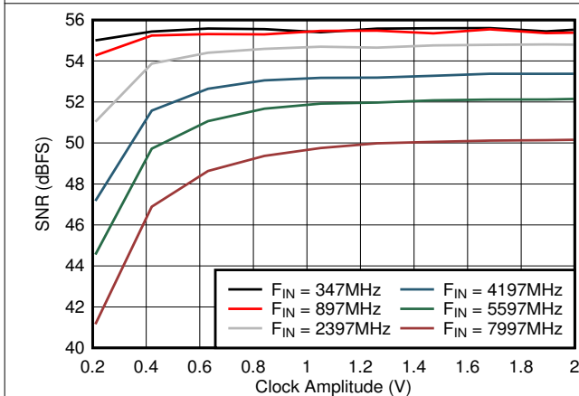
Figure 6-83. Dual Channel Mode: SNR vs Clock Amplitude
