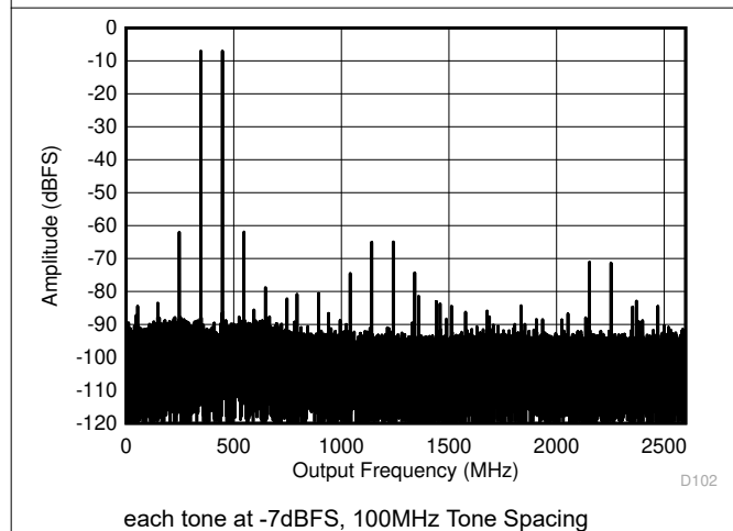
Figure 6-27. DES Mode: Two Tone FFT at 5597MHz
