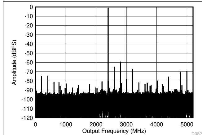
Figure 6-7. DES Mode: Single Tone FFT at 2397MHz
