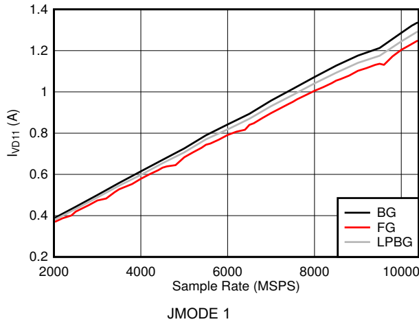
Figure 6-123. DES Mode: I_{VD11} vs Sample Rate
