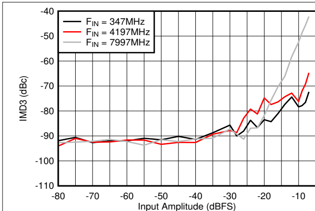
Figure 6-105. Dual Channel Mode: IMD3 vs Input Amplitude
