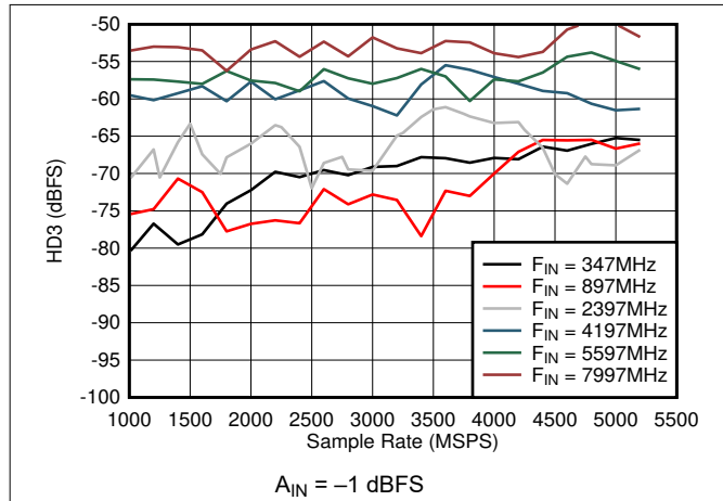
Figure 6-53. Dual Channel Mode: HD3 vs Sample Rate and Input Frequency
