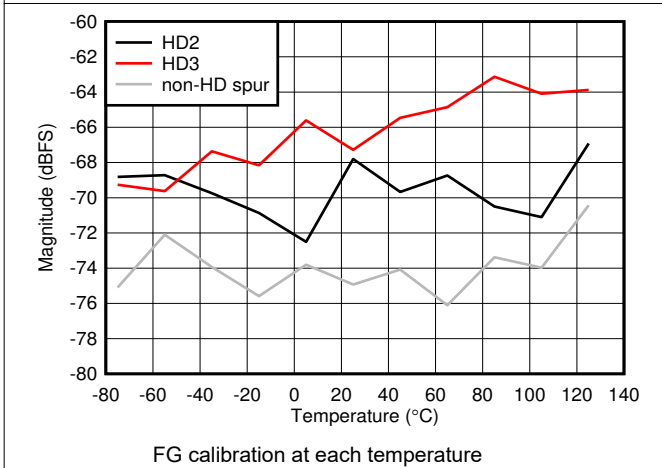
Figure 6-87. DES Mode: HD2, HD3 and Worst non-HD Spur vs Temperature
