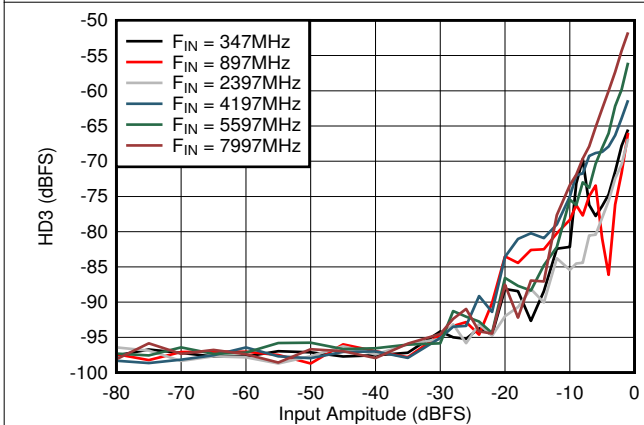
Figure 6-77. Dual Channel Mode: HD3 vs Input Amplitude and Frequency
