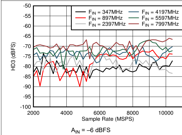
Figure 6-39. DES Mode: HD3 vs Sample Rate and Input Frequency
