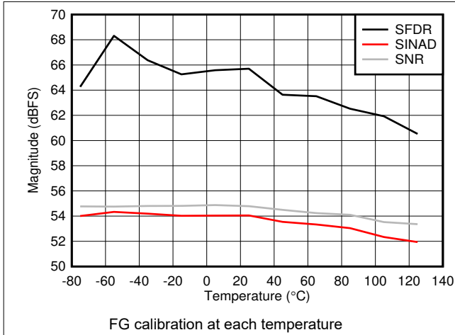
Figure 6-89. Dual Channel Mode: SNR, SINAD and SFDR vs Temperature
