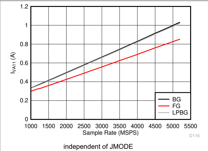
Figure 6-132. Dual Channel Mode: I_{VA11} vs Sample Rate
