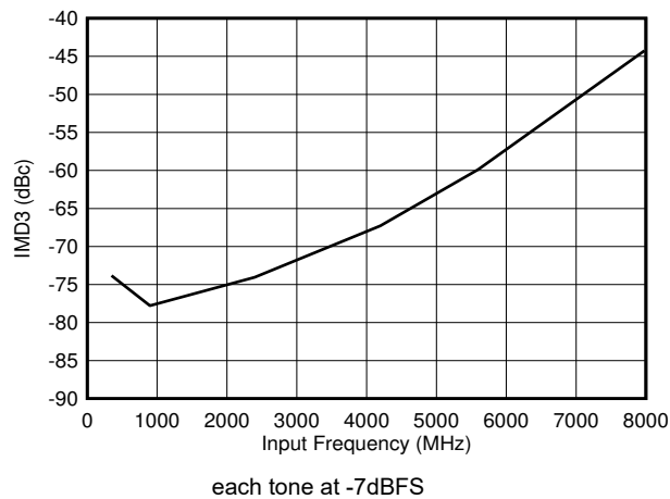
Figure 6-99. DES Mode: IMD3 vs Input Frequency
