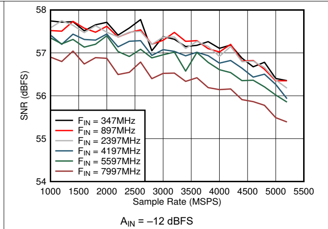
Figure 6-46. Dual Channel Mode: SNR vs Sample Rate and Input Frequency
