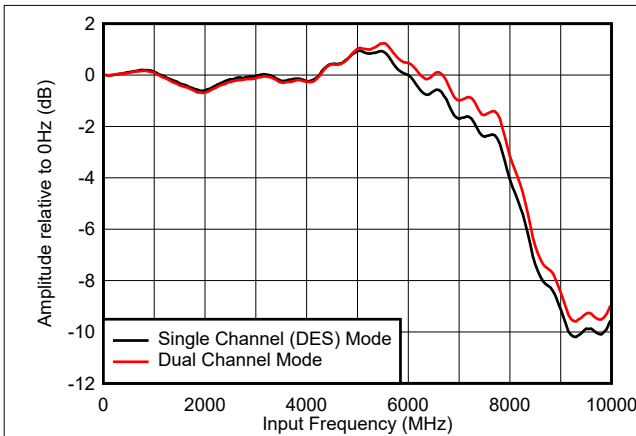
Figure 6-1. Input Amplitude vs Input Frequency
