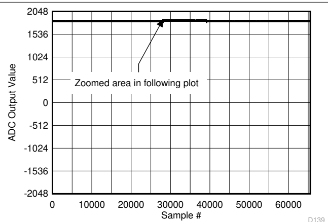
Figure 6-144. Background Calibration Core Transition (DC Signal)
