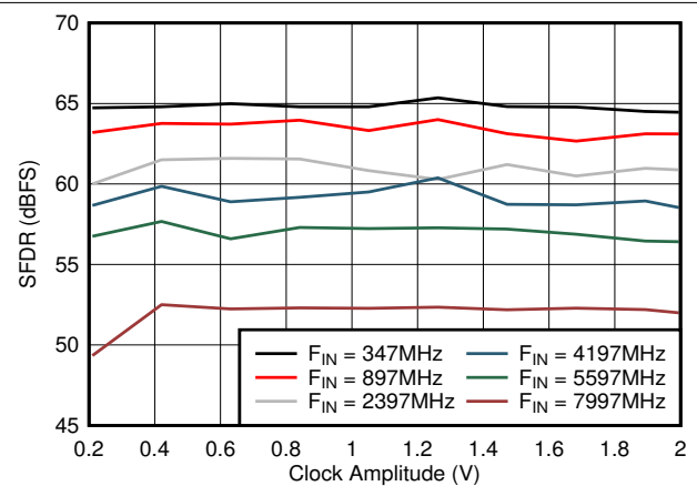
Figure 6-82. DES Mode: SFDR vs Clock Amplitude
