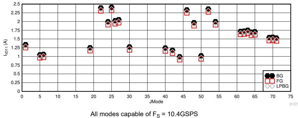
Figure 6-111. DES Mode: I_{VD11} vs JMODE at 10.4GSPS
