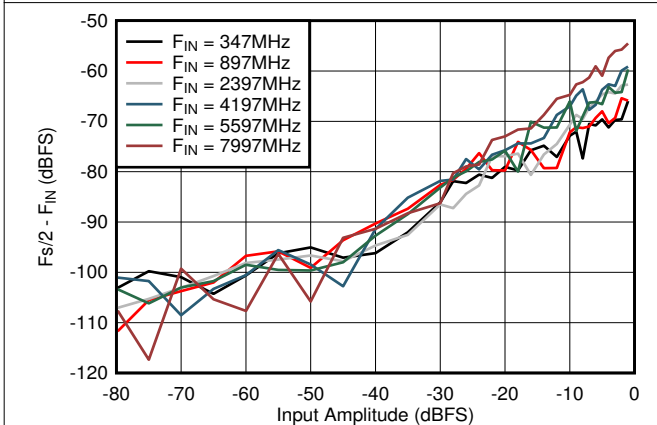
Figure 6-65. DES Mode: F_s/2 - F_{IN} vs Input Amplitude and Frequency
