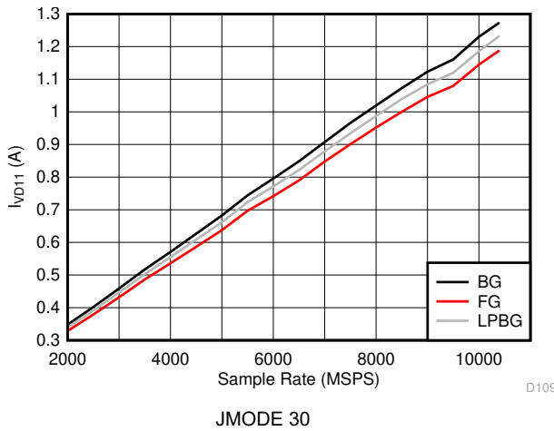
Figure 6-125. DES Mode: I_{VD11} vs Sample Rate
