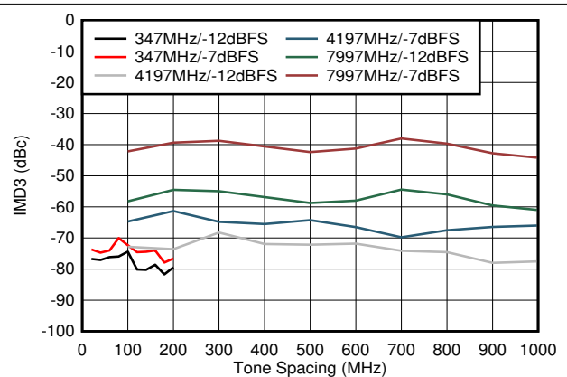
Figure 6-106. Dual Channel Mode: IMD3 vs Tone Spacing
