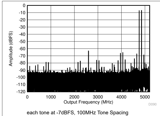
Figure 6-15. DES Mode: Two Tone FFT at 5597MHz
