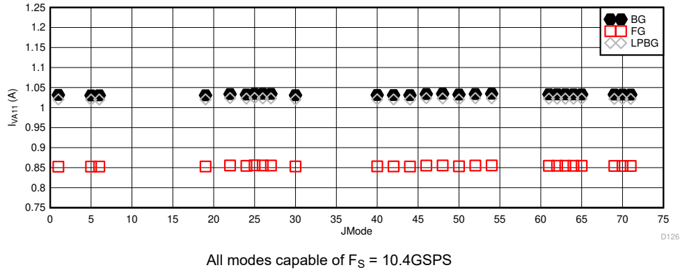
Figure 6-110. DES Mode: I_{VA11} vs JMODE at 10.4GSPS
