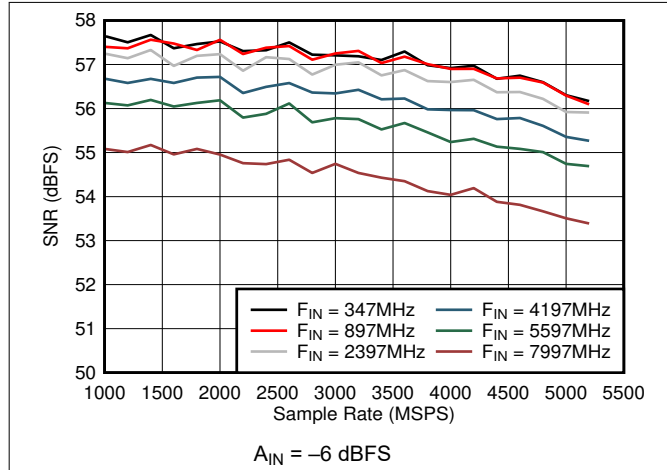
Figure 6-45. Dual Channel Mode: SNR vs Sample Rate and Input Frequency
