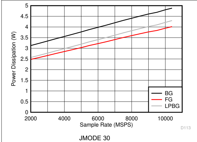
Figure 6-129. DES Mode: Power Dissipation vs Sample Rate
