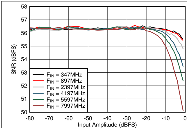
Figure 6-57. DES Mode: SNR vs Input Amplitude and Frequency
