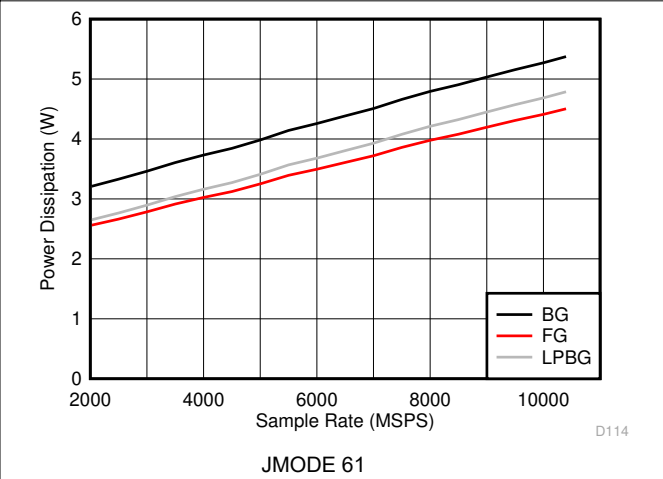
Figure 6-130. DES Mode: Power Dissipation vs Sample Rate
