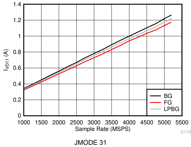
Figure 6-135. Dual Channel Mode: I_{VD11} vs Sample Rate
