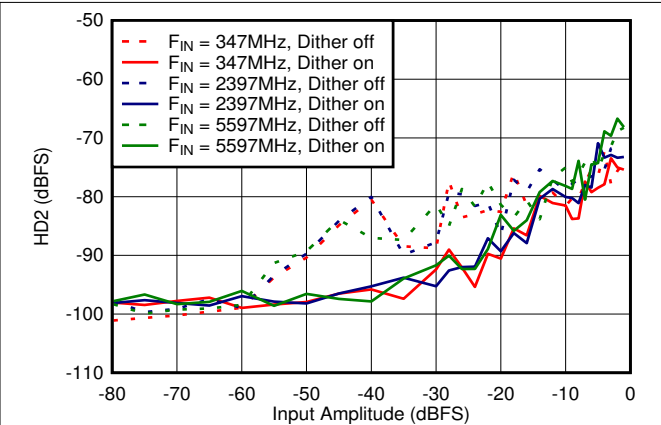
Figure 6-76. Dual Channel Mode: HD2 vs Input Amplitude and Dither
