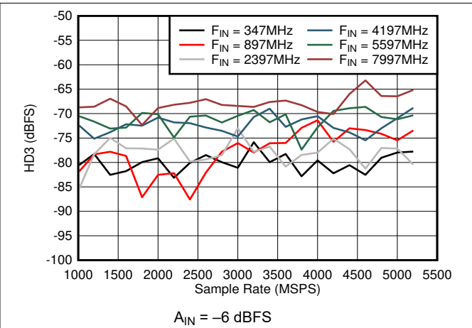
Figure 6-54. Dual Channel Mode: HD3 vs Sample Rate and Input Frequency
