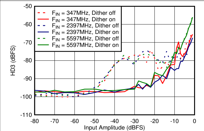
Figure 6-78. Dual Channel Mode: HD3 vs Input Amplitude and Dither
