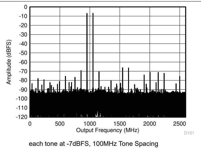
Figure 6-26. DES Mode: Two Tone FFT at 4197MHz
