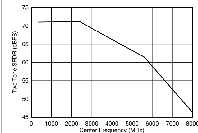
Figure 6-107. Dual Channel Mode: Two Tone SFDR vs Input Frequency
