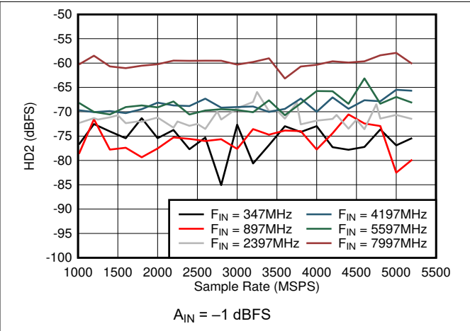
Figure 6-50. Dual Channel Mode: HD2 vs Sample Rate and Input Frequency
