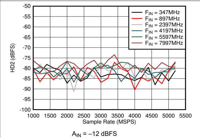
Figure 6-52. Dual Channel Mode: HD2 vs Sample Rate and Input Frequency
