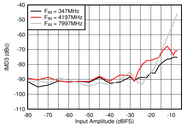
Figure 6-100. DES Mode: IMD3 vs Input Amplitude
