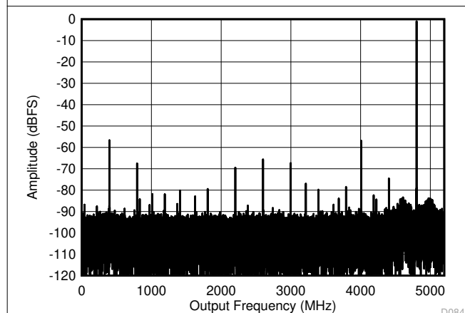
Figure 6-9. DES Mode: Single Tone FFT at 5597MHz
