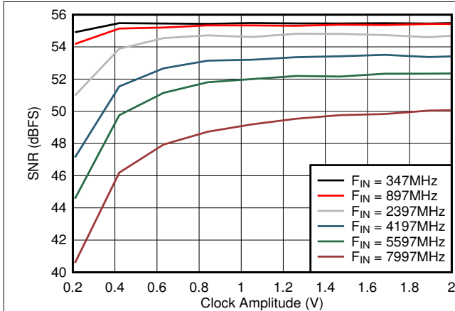
Figure 6-81. DES Mode: SNR vs Clock Amplitude
