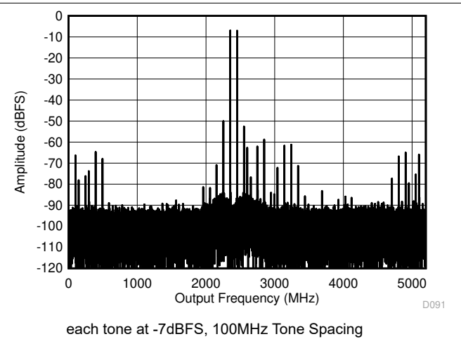
Figure 6-16. DES Mode: Two Tone FFT at 7997MHz
