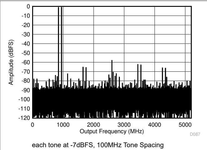
Figure 6-12. DES Mode: Two Tone FFT at 897MHz
