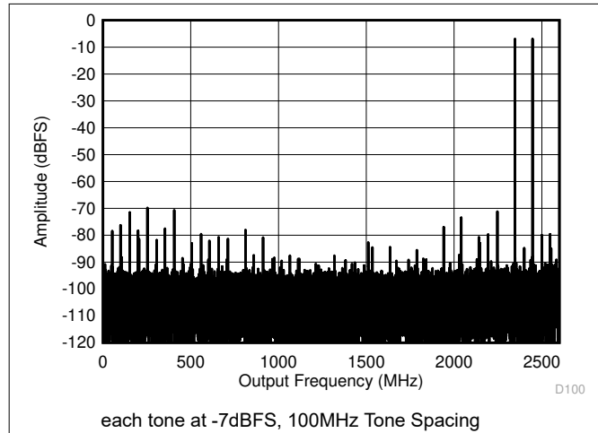
Figure 6-25. DES Mode: Two Tone FFT at 2397MHz
