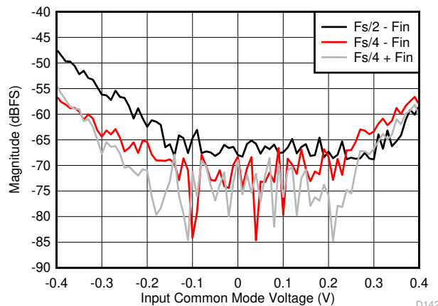
Figure 6-98. F_s/2 - F_{IN} and F_s/4 \pm F_{IN} vs Input Common Mode Voltage
