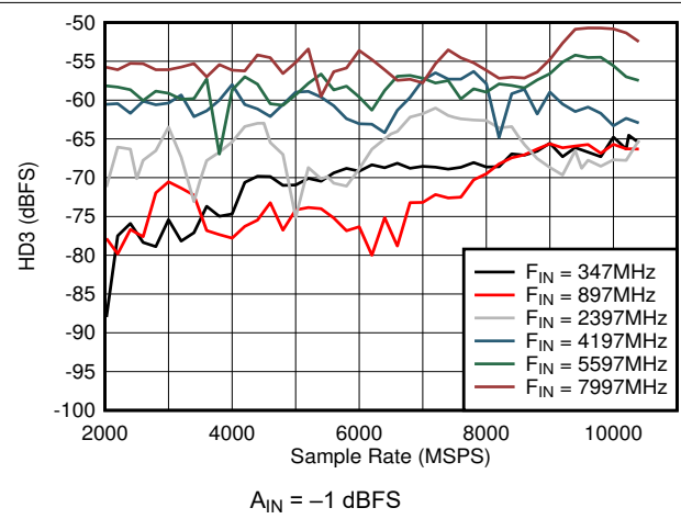
Figure 6-38. DES Mode: HD3 vs Sample Rate and Input Frequency
