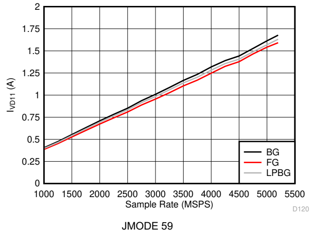
Figure 6-136. Dual Channel Mode: I_{VD11} vs Sample Rate
