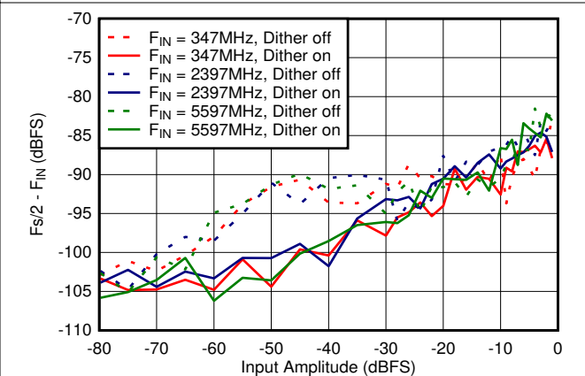
Figure 6-80. Dual Channel Mode: F_s/2 - F_{IN} vs Input Amplitude and Dither
