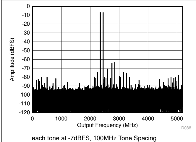
Figure 6-13. DES Mode: Two Tone FFT at 2397MHz
