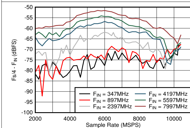
Figure 6-43. DES Mode: F_s/4 - F_{IN} vs Sample Rate and Input Frequency
