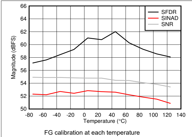
Figure 6-85. DES Mode: SNR, SINAD and SFDR vs Temperature
