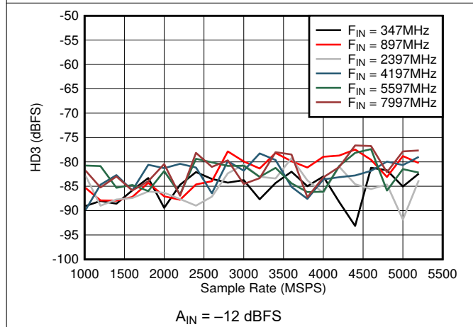
Figure 6-55. Dual Channel Mode: HD3 vs Sample Rate and Input Frequency
