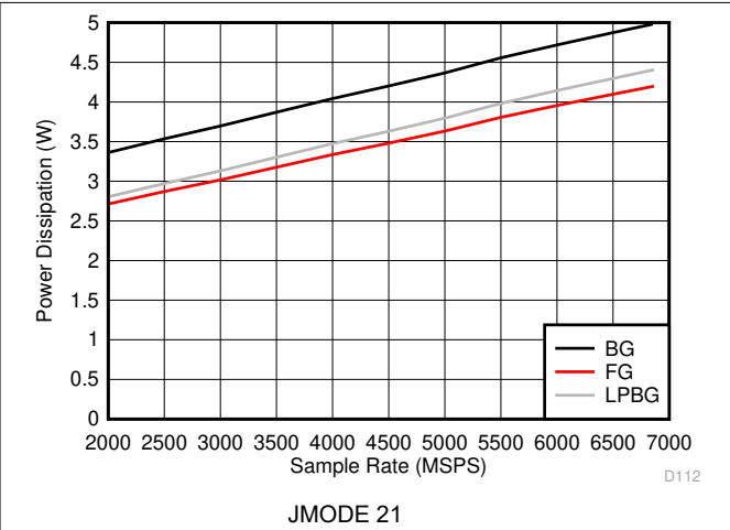
Figure 6-128. DES Mode: Power Dissipation vs Sample Rate
