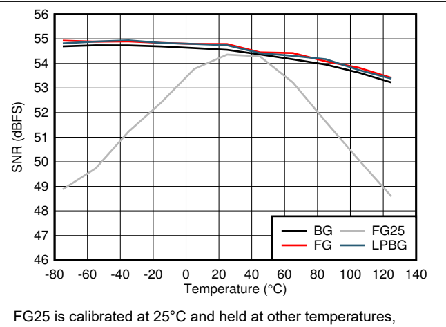
Figure 6-86. DES Mode: SNR vs Temperature and Calibration Mode
