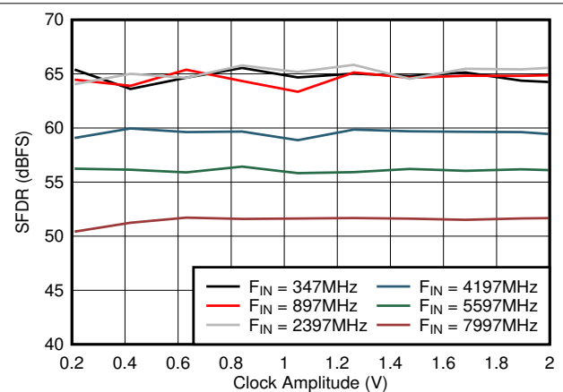
Figure 6-84. Dual Channel Mode: SFDR vs Clock Amplitude
