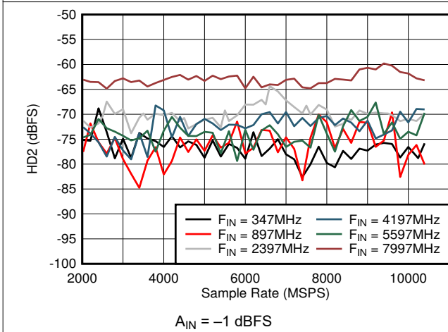
Figure 6-35. DES Mode: HD2 vs Sample Rate and Input Frequency
