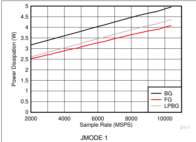
Figure 6-127. DES Mode: Power Dissipation vs Sample Rate
