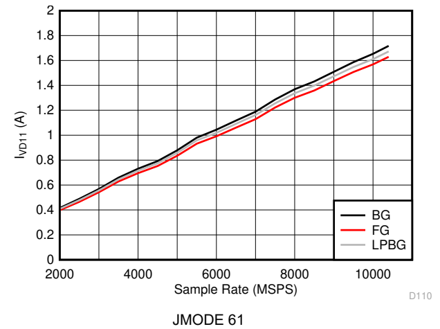
Figure 6-126. DES Mode: I_{VD11} vs Sample Rate
