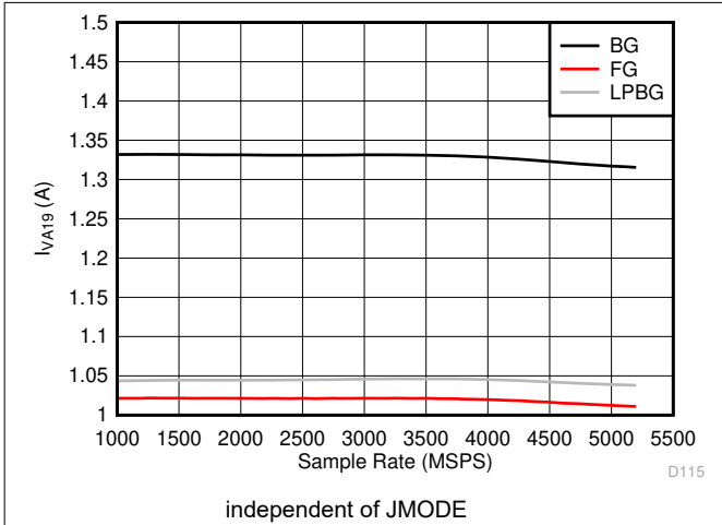
Figure 6-131. Dual Channel Mode: I_{VA19} vs Sample Rate
