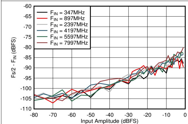
Figure 6-79. Dual Channel Mode: F_s/2 - F_{IN} vs Input Amplitude and Frequency
