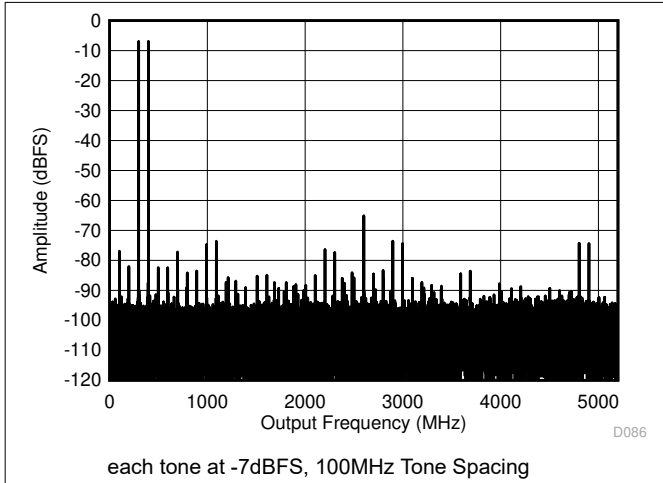
Figure 6-11. DES Mode: Two Tone FFT at 347MHz
