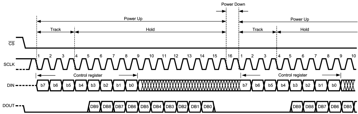
ADC104S021 Operational Timing Diagram
