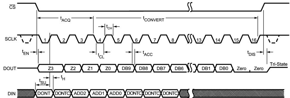
ADC104S021 Serial Timing Diagram
