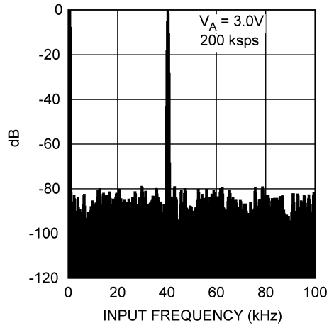
Spectral Response - 3V, 200 kSPS
