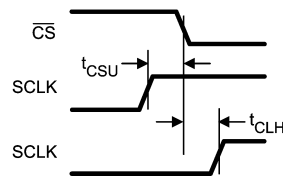
SCLK and CS Timing Parameters
