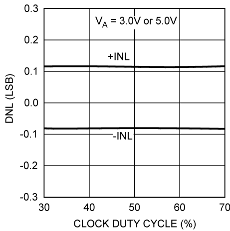
DNL vs. Clock Duty Cycle
