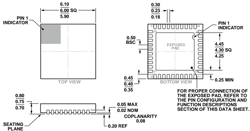
Figure 77. 40-Lead Lead Frame Chip Scale Package [LFCSP_WQ] 6 mm × 6 mm Body, Very Very Thin Quad (CP-40-10) Dimension shown in millimeters
