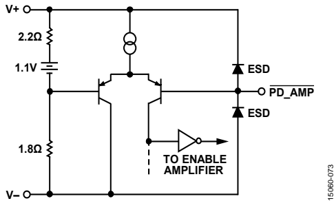
Figure 61. Shutdown Circuit
