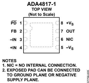
Figure 5. ADA4817-1 Pin Configuration (8-Lead LFCSP)
