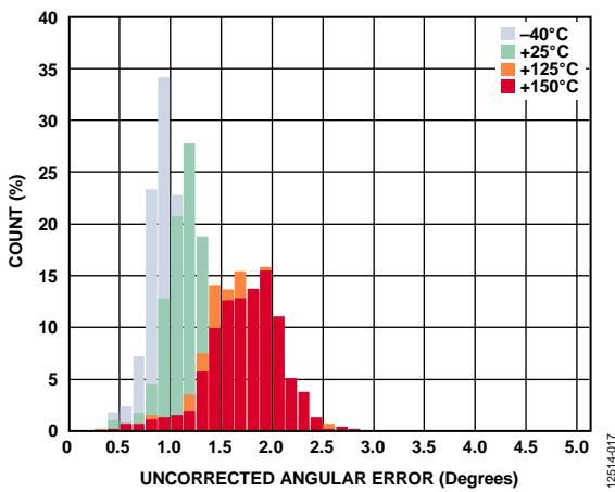
Figure 10. Uncorrected Angular Error, V_{DD} = 5.5\text{ V} , GC = \text{Off}
