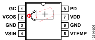
Figure 25. Bonding Arrangement and Sensor Alignment in Package
