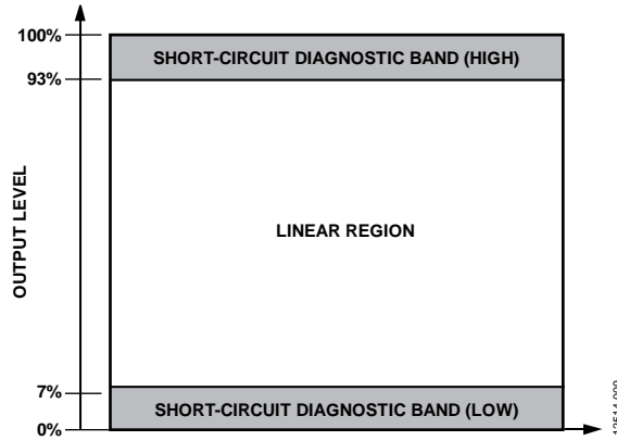
Figure 34. Output Span Classification During Short-Circuit Diagnostic Condition
