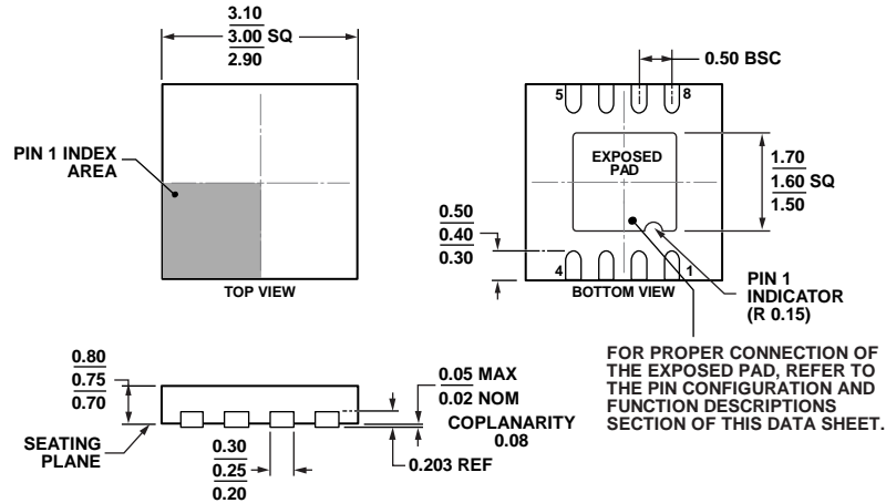
Figure 75. 8-Lead Lead Frame Chip Scale Package [LFCSWP] 3 mm x 3 mm Body, Very Very Thin, Dual Lead (CP-8-12)
