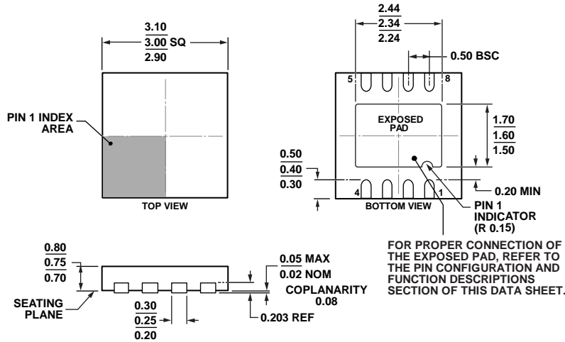
Figure 76. 8-Lead Lead Frame Chip Scale Package [LFCSP_WD] 3 mm x 3 mm Body, Very Very Thin, Dual Lead (CP-8-11) Dimensions shown in millimeters
