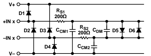
Figure 72. Input EMI Filter and Clamp Circuit
