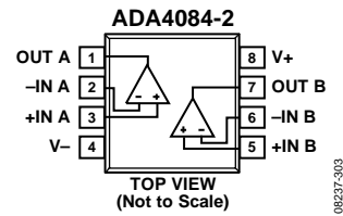
Figure 7. ADA4084-2, 8-Lead SOIC (R)
