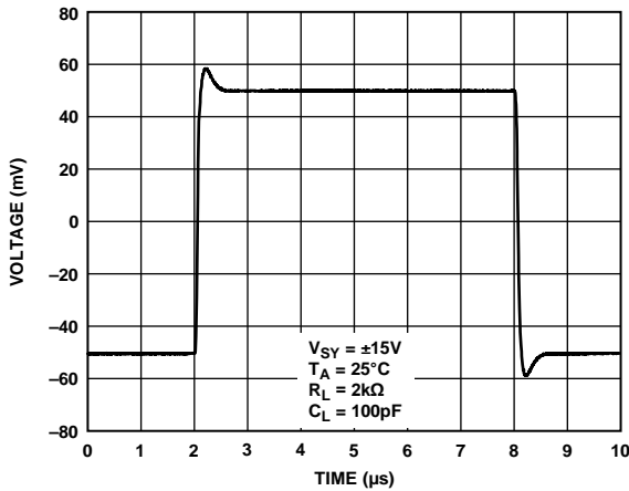
Figure 91. Small Signal Transient Response
