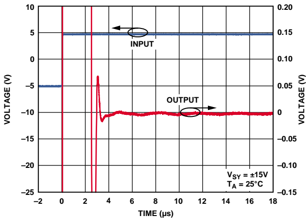
Figure 92. Settling Time
