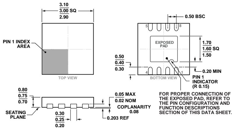
Figure 115. 8-Lead Lead Frame Chip Scale Package [LFCSF_WD] 3 mm x 3 mm Body, Very Very Thin, Dual Lead (CP-8-12)
