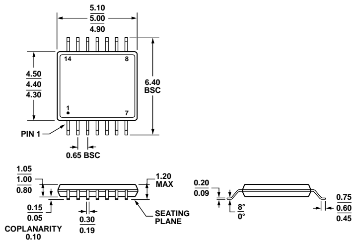
Figure 117. 14-Lead Thin Shrink Small Outline Package [TSSOP] (RU-14) Dimensions shown in millimeters
