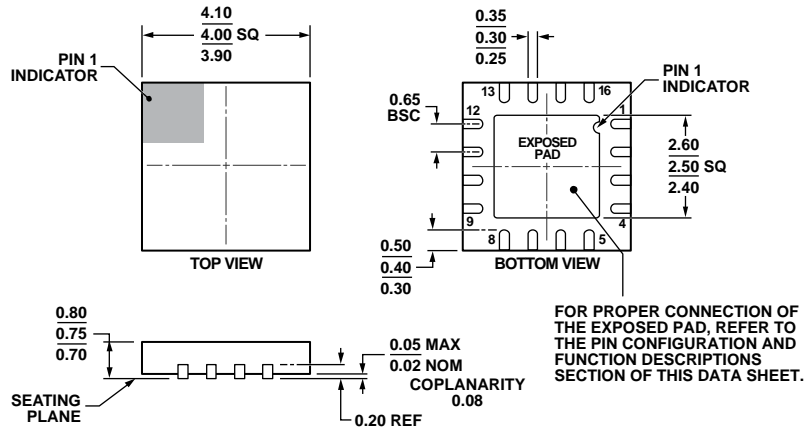
Figure 116. 16-Lead Lead Frame Chip Scale Package [LF CSP_WQ] 4 mm × 4 mm Body, Very Very Thin Quad (CP-16-26) Dimensions shown in millimeters
