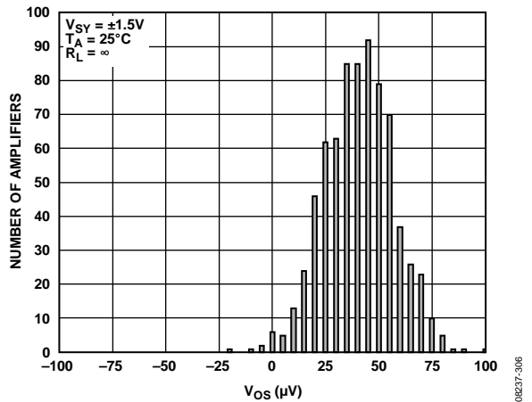
Figure 11. Input Offset Voltage ( V_{os} ) Distribution, SOT-23
