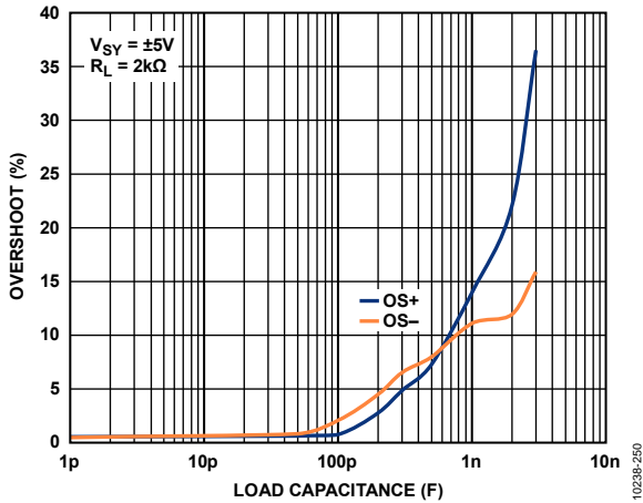
Figure 53. Small Signal Overshoot vs. Load Capacitance, V_{SV} = \pm 5 V
