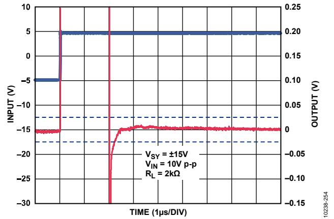
Figure 57. Positive 0.1% Settling Time, V_{SV} = \pm 15 V
