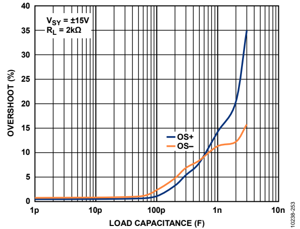
Figure 56. Small Signal Overshoot vs. Load Capacitance, V_{SV} = \pm 15 V
