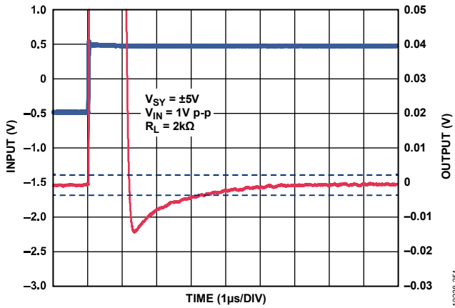
Figure 54. Positive 0.1% Settling Time, V_{SV} = \pm 5 V
