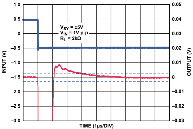
Figure 55. Negative 0.1% Settling Time, V_{SV} = \pm 5 V
