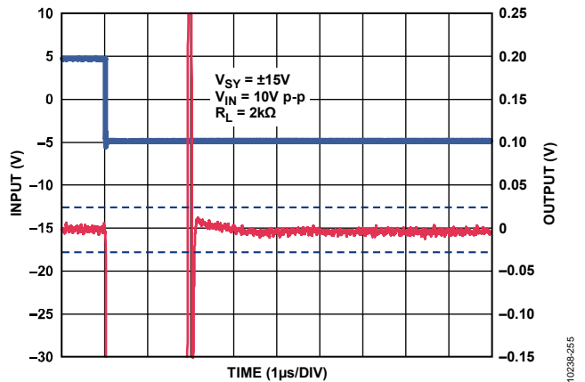
Figure 58. Negative 0.1% Settling Time, V_{SV} = \pm 15 V
