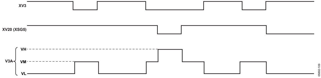
Figure 58. XV3, XV20, and V3A Output Polarities
