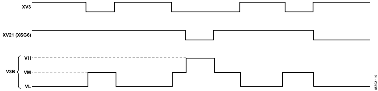
Figure 59. XV3, XV21, and V3B Output Polarities
