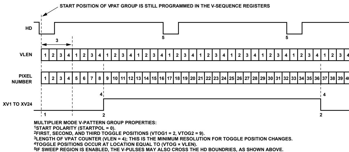
Figure 51. Example of Multiplier Region for Wide Vertical Pulse Timing
