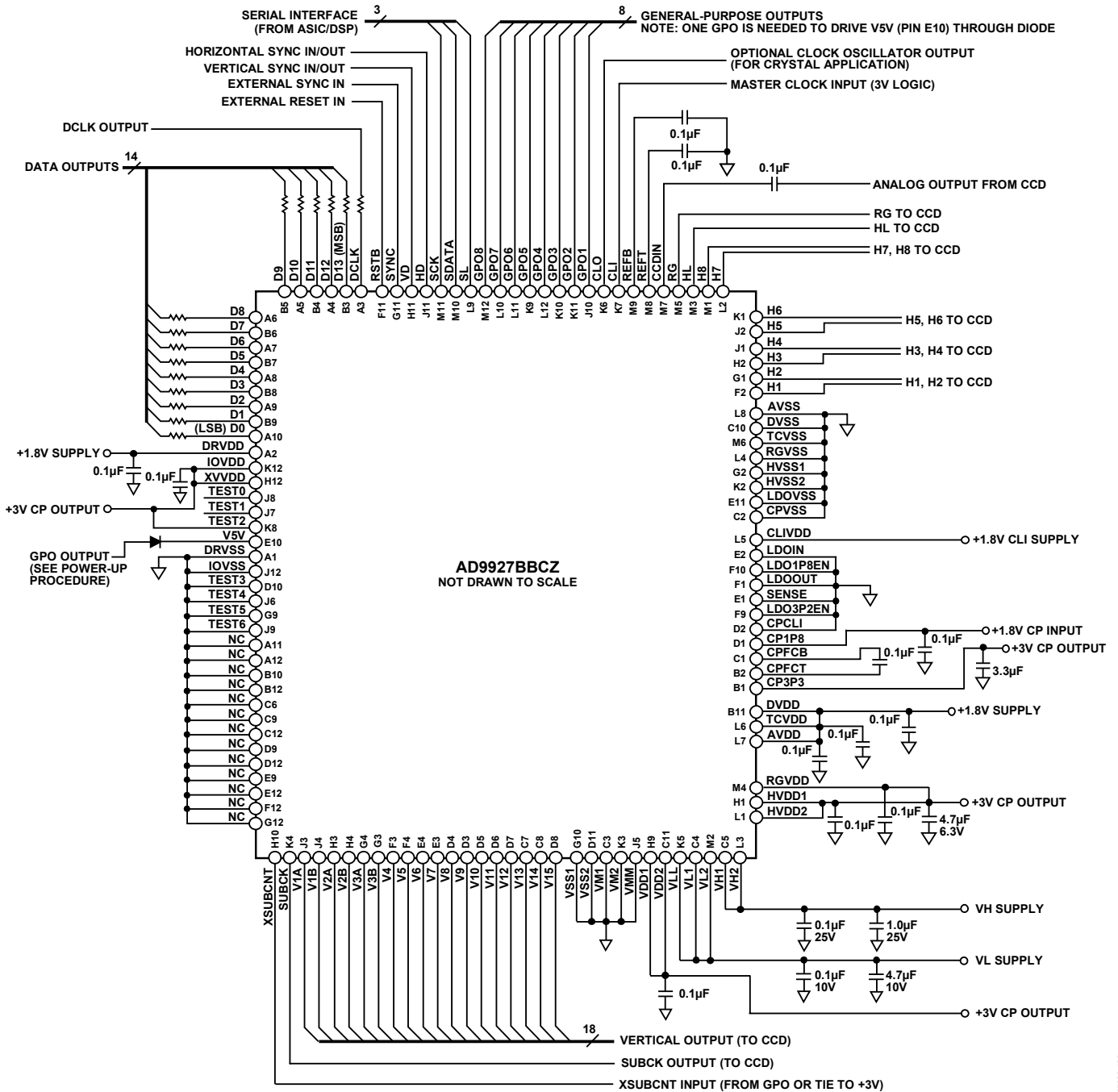
Figure 95. Typical 1.8 V Circuit Configuration Using Charge Pump for HVDD and RGVD
