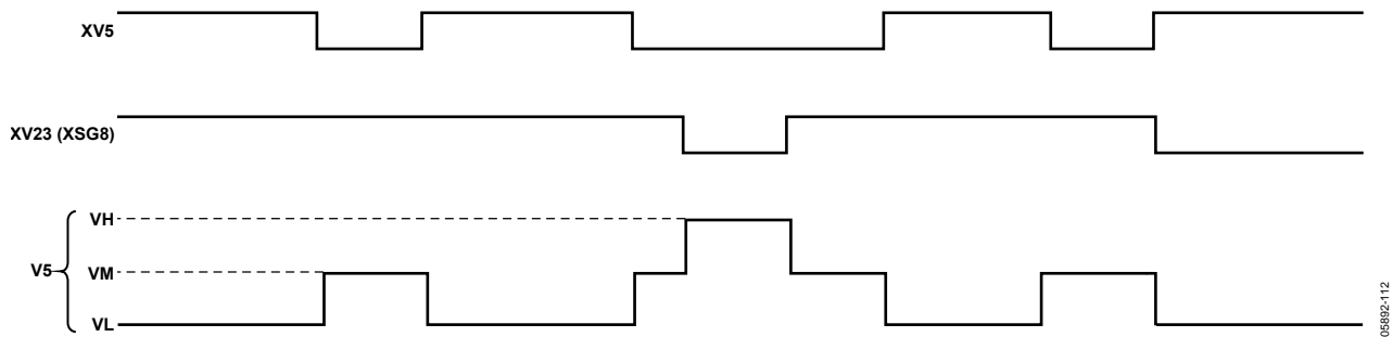
Figure 61. XV5, XV23, and V5 Output Polarities
