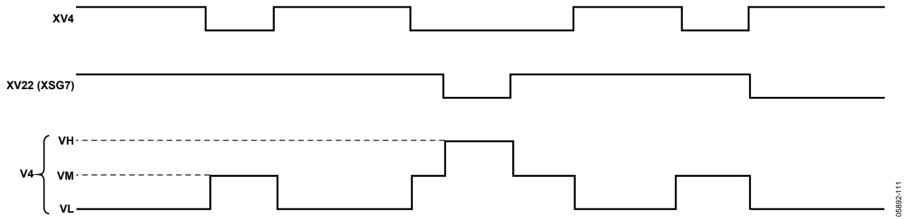
Figure 60. XV4, XV22, and V4 Output Polarities
