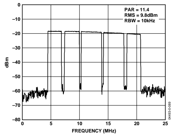
Figure 44. Spectral Plot of 84-Carrier OFDM Test Vector Using IAMPN in Voltage-Mode Configuration with AV_{DD} = 3.3 V (PBR951 Transistors, IAMP Settings of I = 6 mA, N = 2 , G = 6 )
