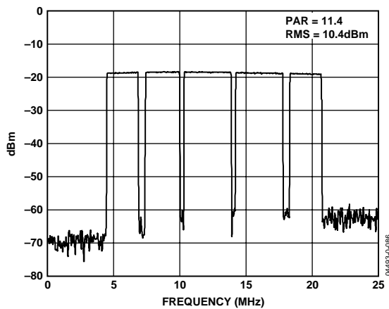
Figure 41. Spectral Plot of 84-Carrier OFDM Test Vector Using IAMPN in Voltage-Mode Configuration with AV_{DD} = 5 V (PBR951 Transistors, IAMP Settings of I = 6 mA, N = 2 , G = 6 )
