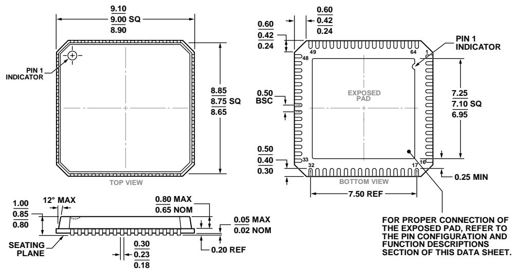
Figure 85. 64-Lead Lead Frame Chip Scale Package (LFCSP) 9 mm x 9 mm and 0.85 mm Package Height [CP-64-3] Dimensions shown in millimeters
