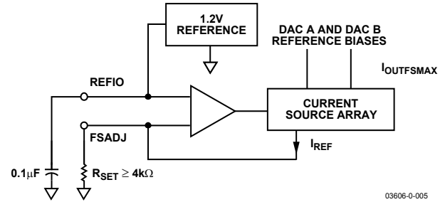
Figure 74. Reference Circuitry
