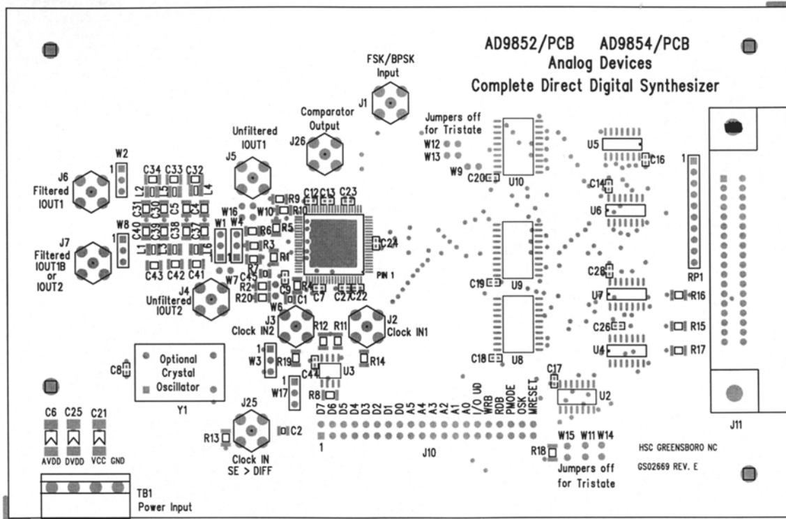
Figure 66. Assembly Drawing
