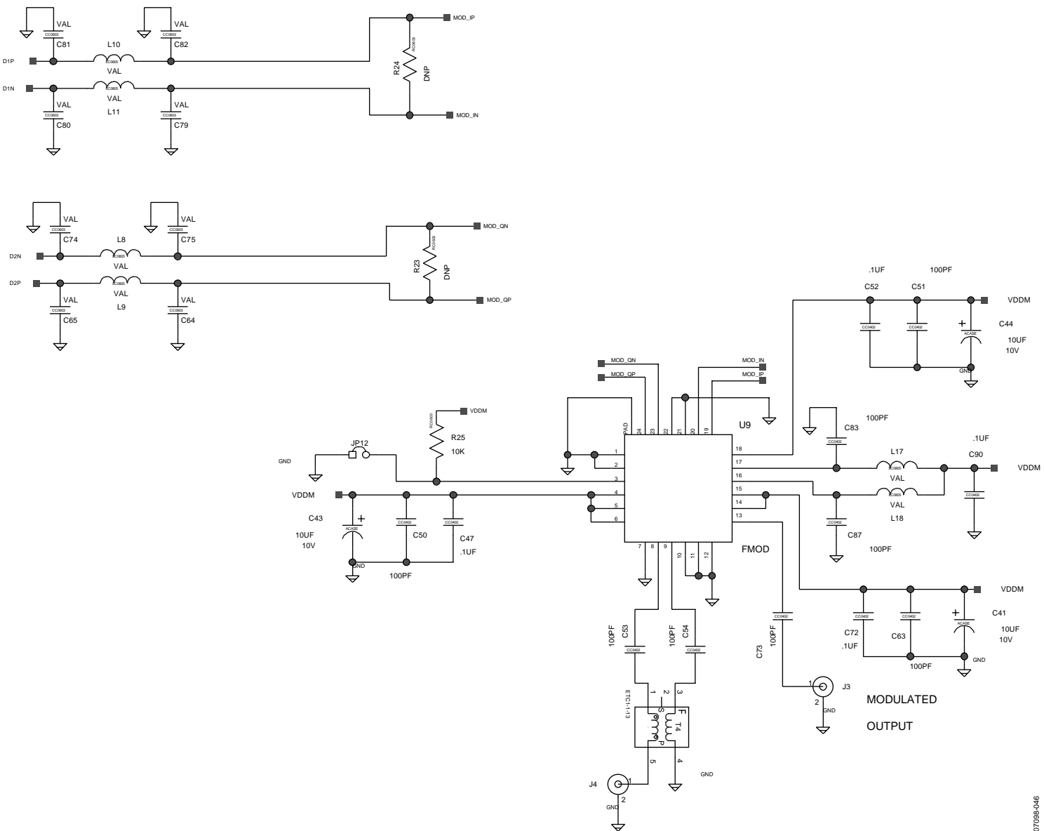
Figure 83. Evaluation Board, ADL5372 (FMOD2) Quadrature Modulator
