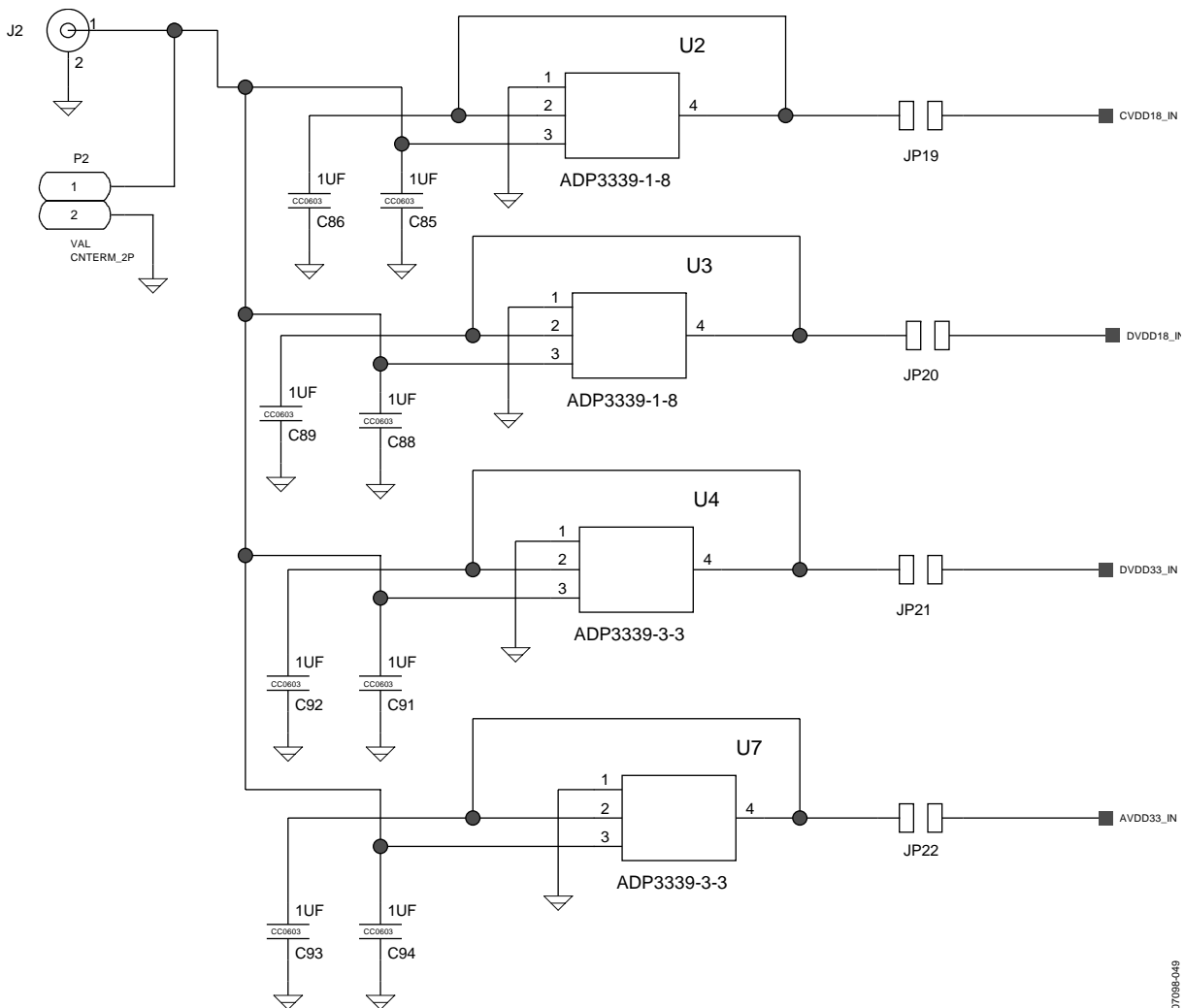
Figure 86. Evaluation Board, On-Board Power Supply
