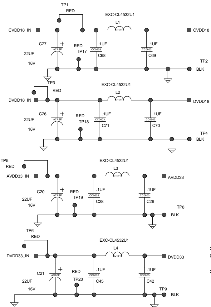
Figure 81. Evaluation Board, Power Supply and Decoupling
