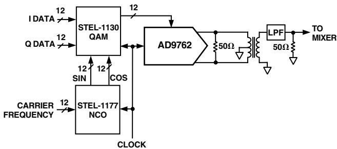
Figure 58. Digital QAM Architecture
