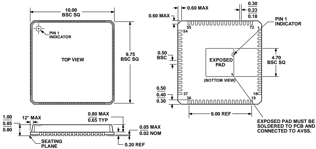
COMPLIANT TO JEDEC STANDARDS MO-220-VNND-3 Figure 44. 72-Lead Lead Frame Chip Scale Package [LFCSP_VQ] 10 mm × 10 mm, Very Thin Quad (CP-72-1) Dimensions shown in millimeters
