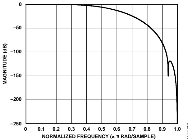
Figure 76. HB4 Filter Response
