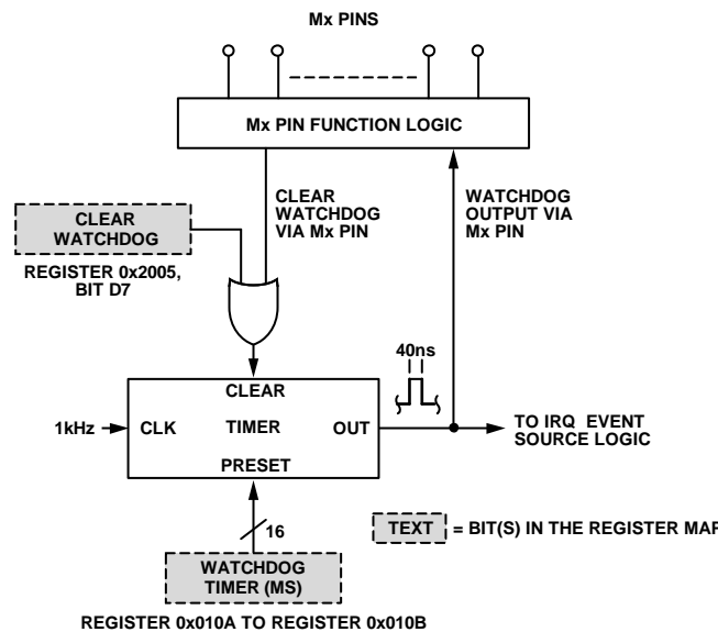
Figure 48. Watchdog Timer
