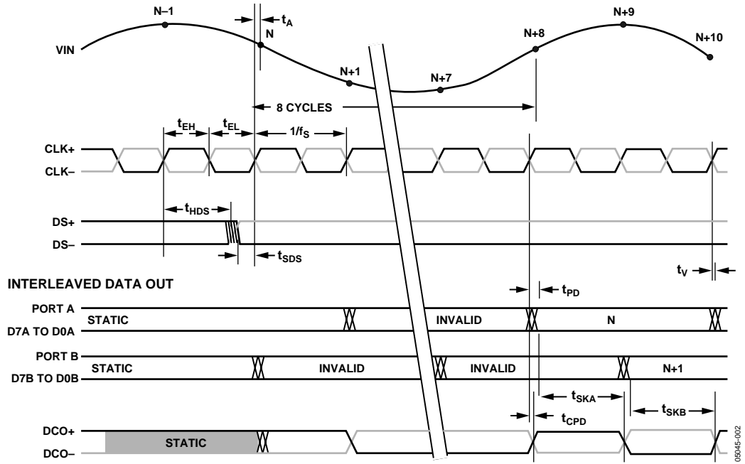
Figure 2. Timing Diagram
