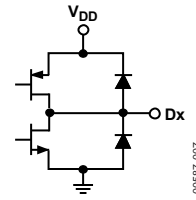
Figure 24. Digital Output Circuit
